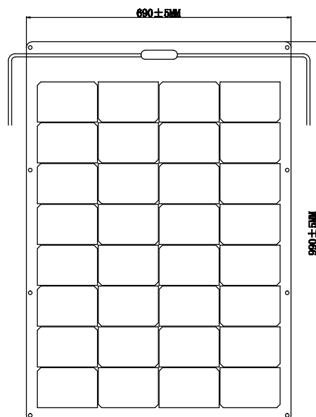
MECHANICAL DRAWINGS
