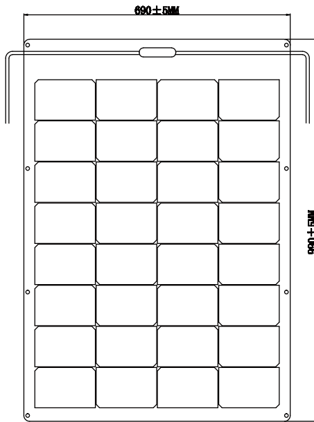
MECHANICAL DRAWINGS
